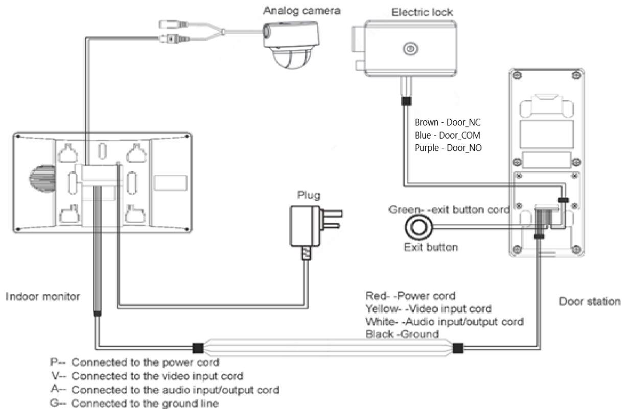
Figure 3-2 Wiring (1)
