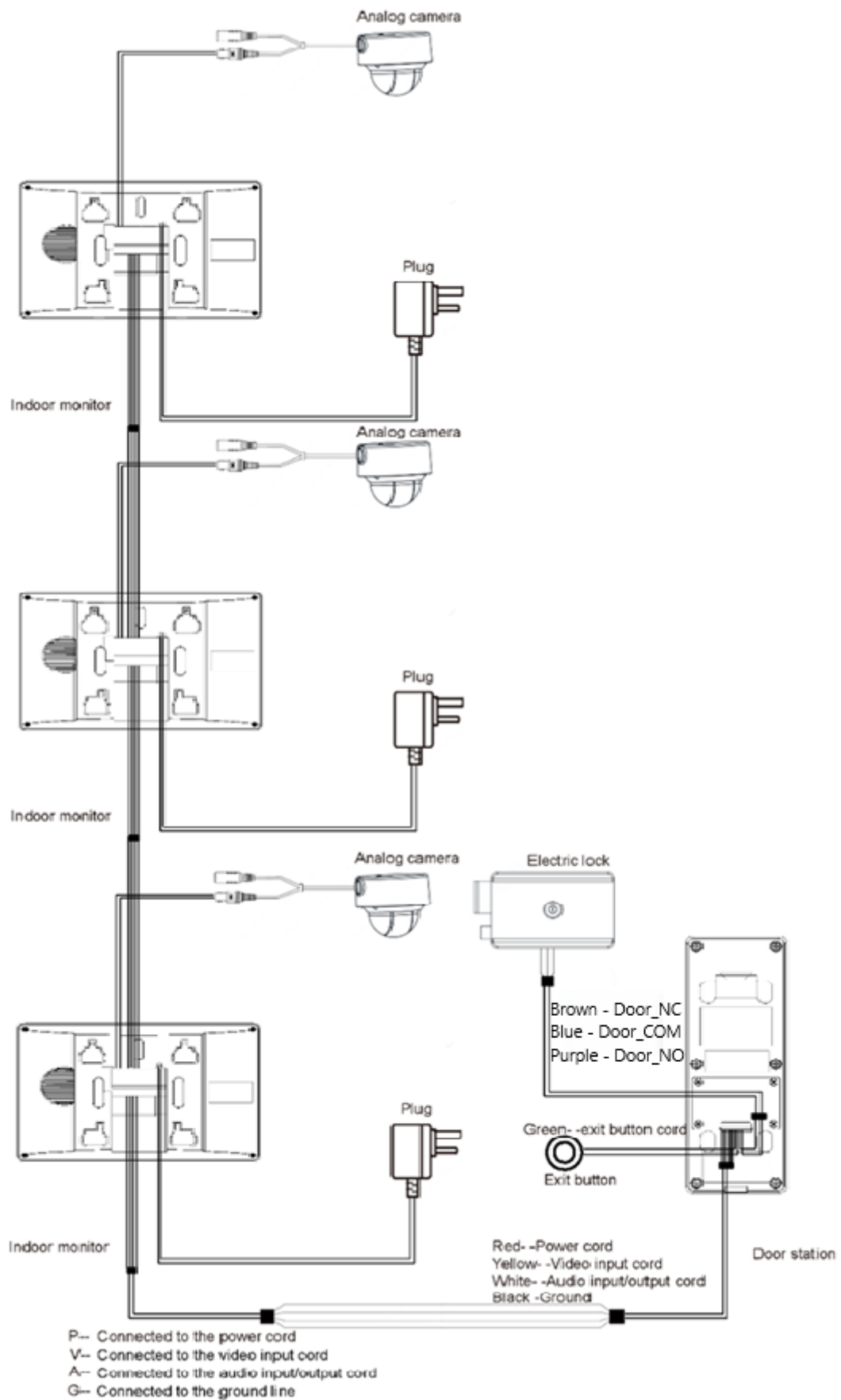
Figure 3-3 Wiring (2)
