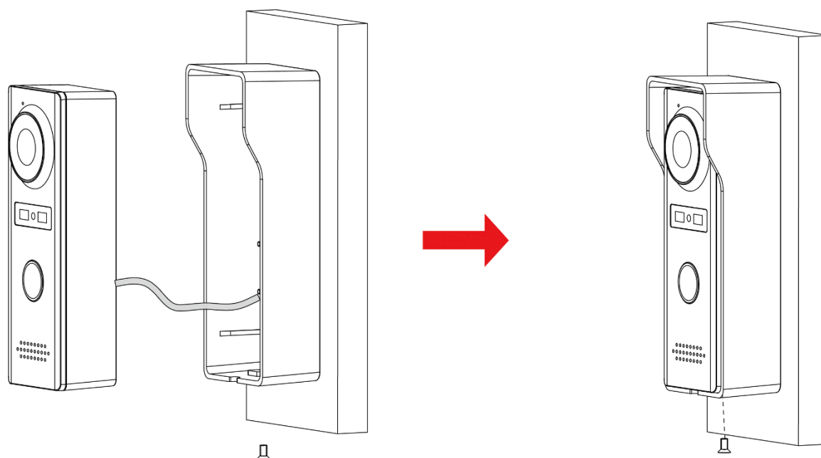
Figure 2-2 VTO installation
