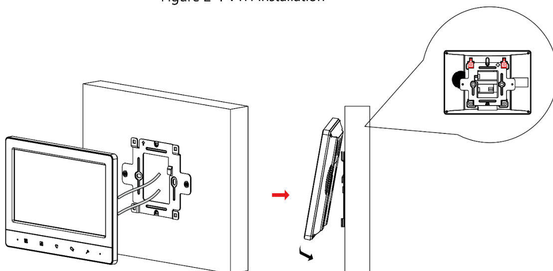
Figure 2-1 VTH installation
